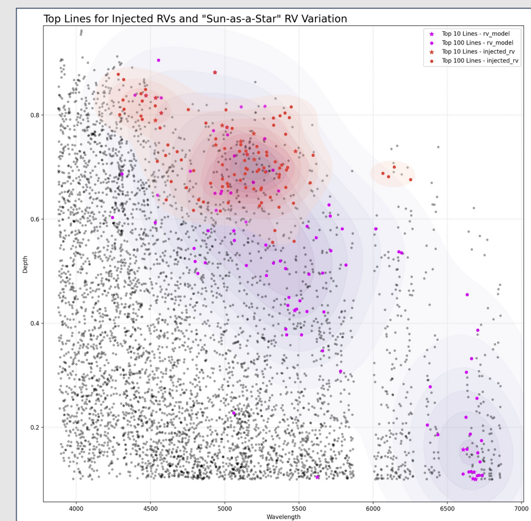
Figure 4: Each spectral line from HARPS-N spectra was input to a CNN targeting an injected planetary RV (red) and separately the “sun-as-a-star” RV variation (purple). The top 100 top performing lines for each trial are highlighted.
